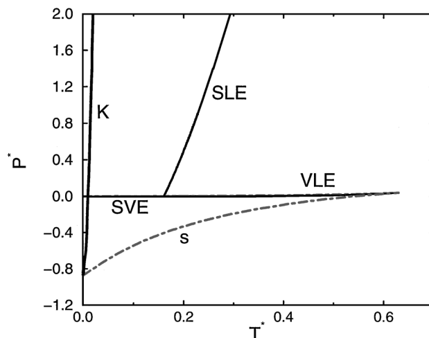
FIG. 16. Calculated phase diagram of the r^{-9} soft-sphere plus mean-field model, showing the vapor-liquid (VLE), solid-liquid (SLE), and solid-vapor (SVE) coexistence loci, the superheated liquid spinodal (s), and the Kauzmann locus (K) in the pressure-temperature plane ( P^* = P\sigma^3/\varepsilon ; T^* = k_B T/\varepsilon ). The Kauzmann locus gives the pressure-dependent temperature at which the entropies of the supercooled liquid and the stable crystal are equal. Note the convergence of the Kauzmann and spinodal loci at T = 0 . See Debenedetti et al. (1999) for details of this calculation.
