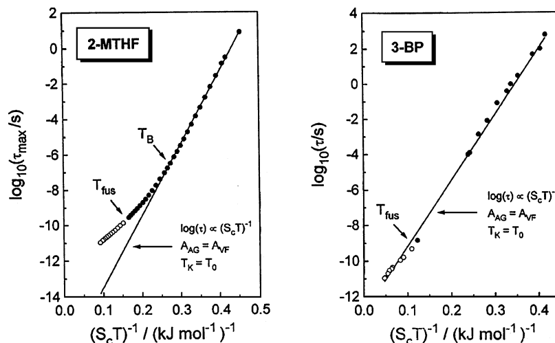
FIG. 12. Adam-Gibbs plots of the dielectric relaxation time of 2-methyltetrahydrofuran (2-MTHF) and 3-bromopentane (3-BP) versus (T_{\text{conf}})^{-1} . The lines are VTF fits, T_{\text{fus}} is the fusion temperature, and T_B is the temperature below which the VTF equation applies. A_{AG} and A_{VF} are prefactors in the Adam-Gibbs and VTF equations, respectively. T_K is the calorimetrically determined Kauzmann temperature, and T_0 is the VTF singular temperature, which were set equal in the VTF (line) fits. (Reprinted with permission from R. Richert and C. A. Angell. Dynamics of glass-forming liquids. V. On the link between molecular dynamics and configurational entropy. J. Chem. Phys. (1998); 108:9016. Copyright © 1998, American Institute of Physics.)
